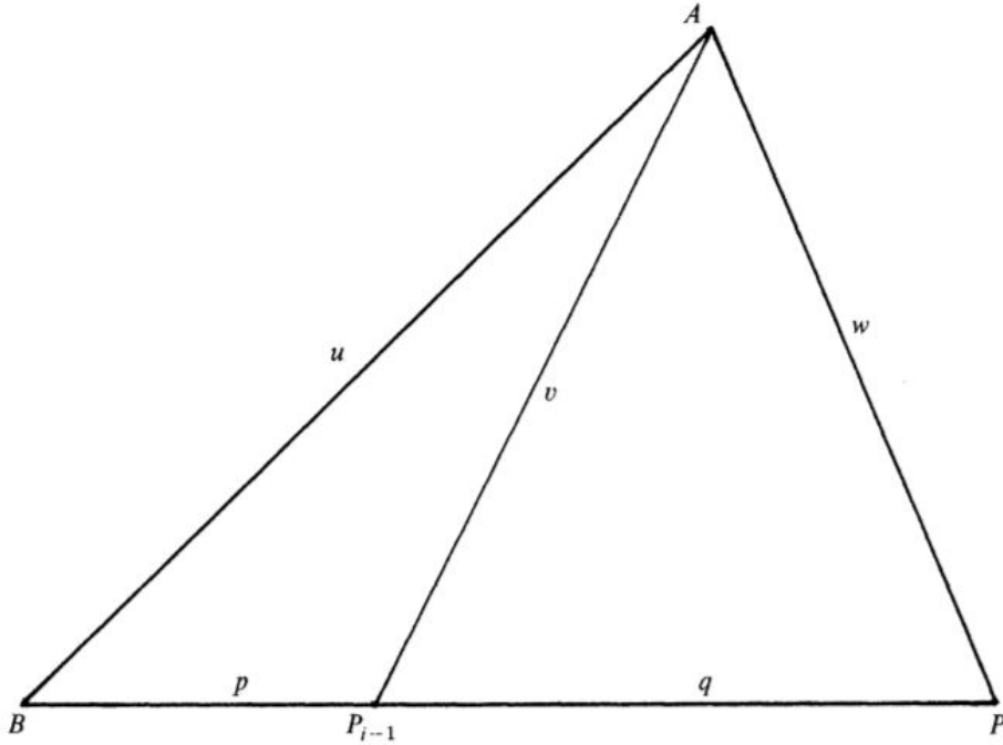
FIGURE 2. Stewart's theorem.
